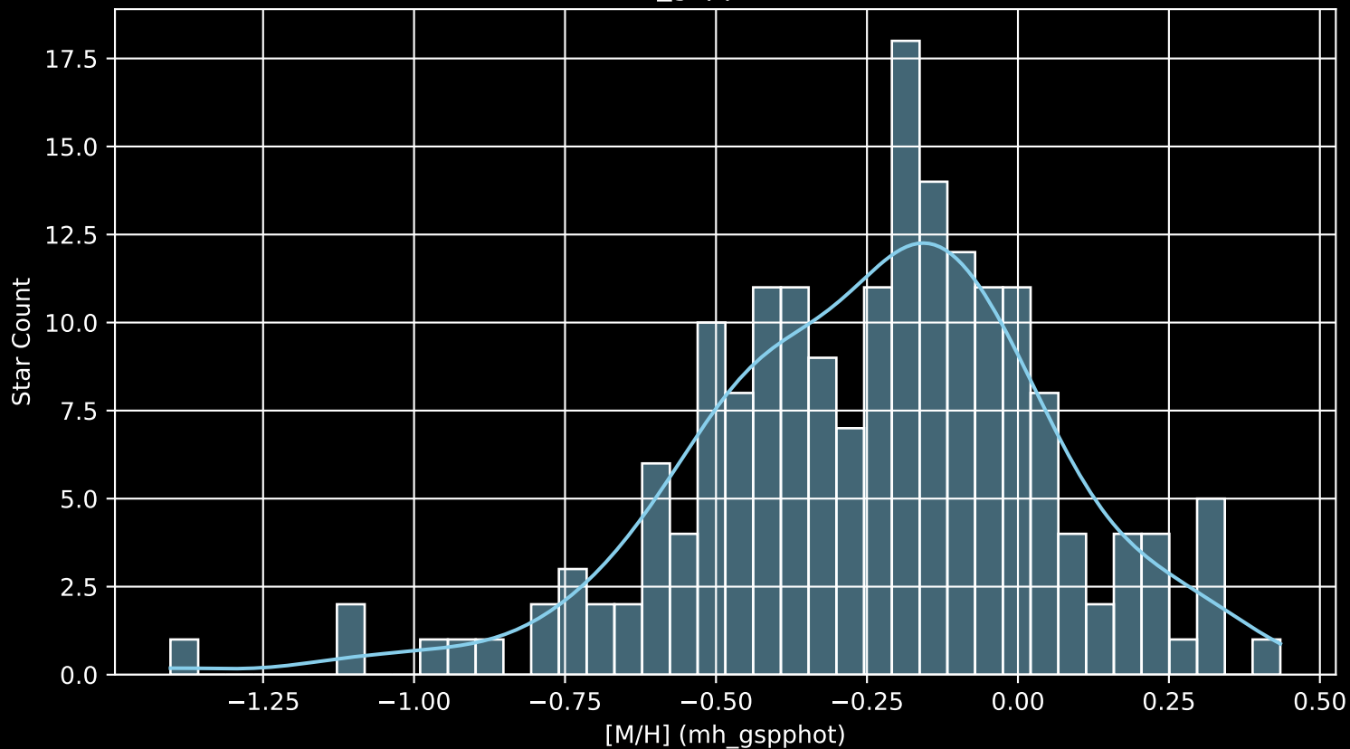
APOGEE DR17 Field: [228+29_MGA [M/H] (mh_gspphot) (n= 187)
