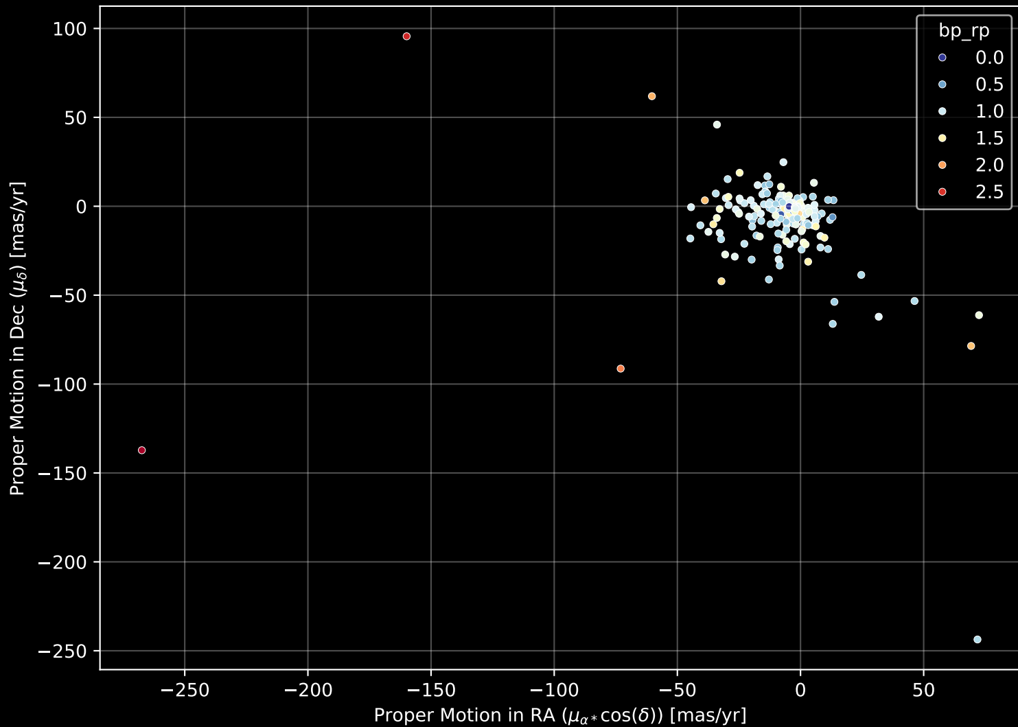
APOGEE DR17 Field: [228+29_MGA] Proper Motion Diagram (n= 190)
