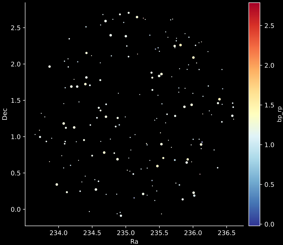
APOGEE DR17 Field: [228+29_MGA] Stars: 190
