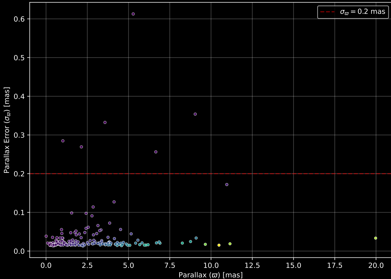
APOGEE DR17 Field: [228+29_MGA] Parallax Quality (n= 190)
