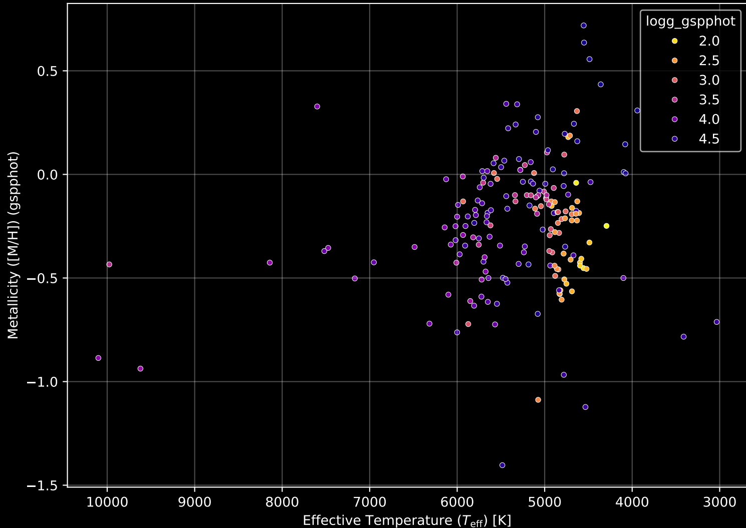
APOGEE DR17 Field: [228+29_MGA] Stellar Population Parameters (n= 190)
