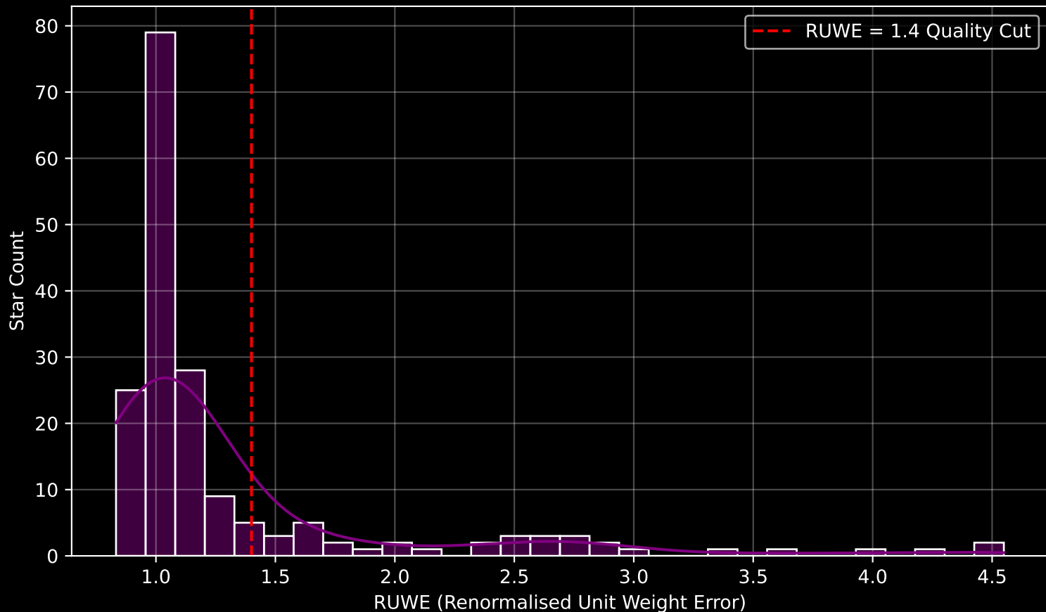
GAPOGEE DR17 Field [228+29_MGA] RUWE Distribution (n= 180)
