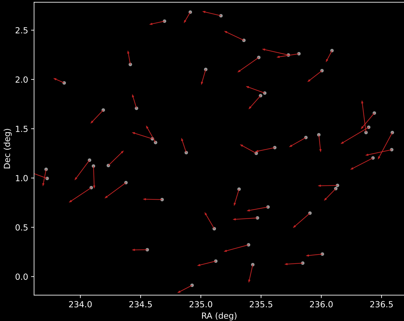
APOGEE DR17 Cluster 6 Proper Motion Vectors (n=51)
