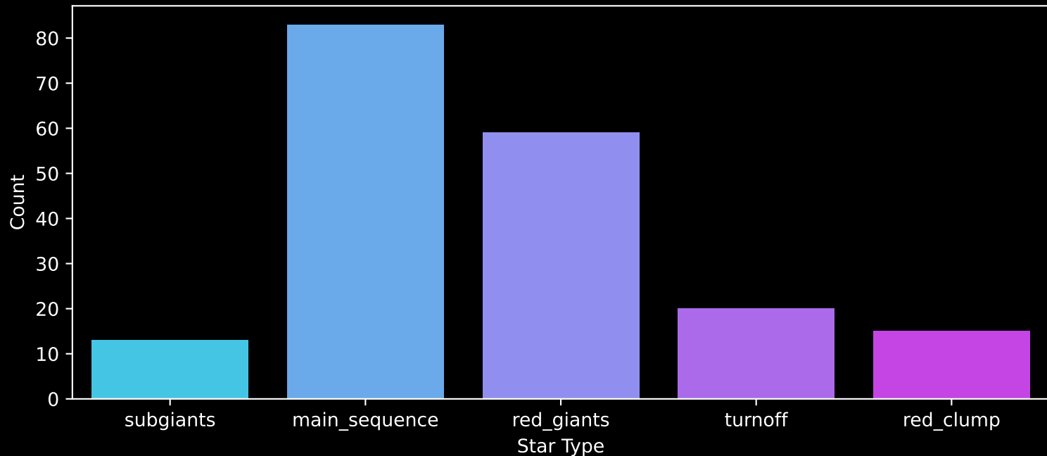
APOGEE DR17 Field: [228+29_MGA] Count plot of Star Type
